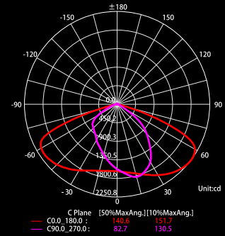
C plane lighting distributions
