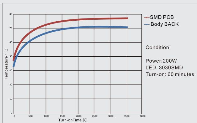
Temperature Rise
